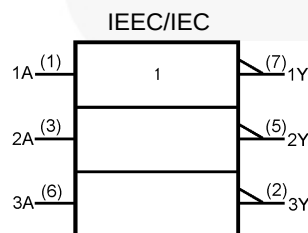
Figure 1. Logic Symbol
